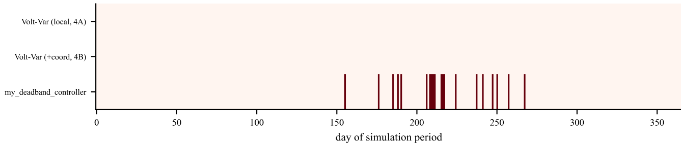
S4-RPi HIL — violation presence (red = \geq 1 violation that day)
